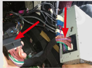
19. Plug android male connector to CD, Connect original harness to android female connector.
