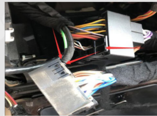
18. Relocate optic cables from original male socket into android male socket.
